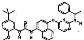
1-(5-tert-Butyl-2-methoxy-phenyl)-3-{4-[2-(1-phenylethylamino)-pyrimidin-4-yloxy]-naphthalen-1-yl}-urea;
